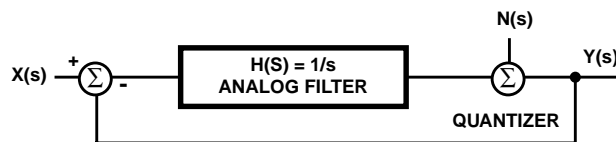
FIGURE 8. LINEARIZED MODEL OF 1ST ORDER SIGMA DELTA MODULATOR
