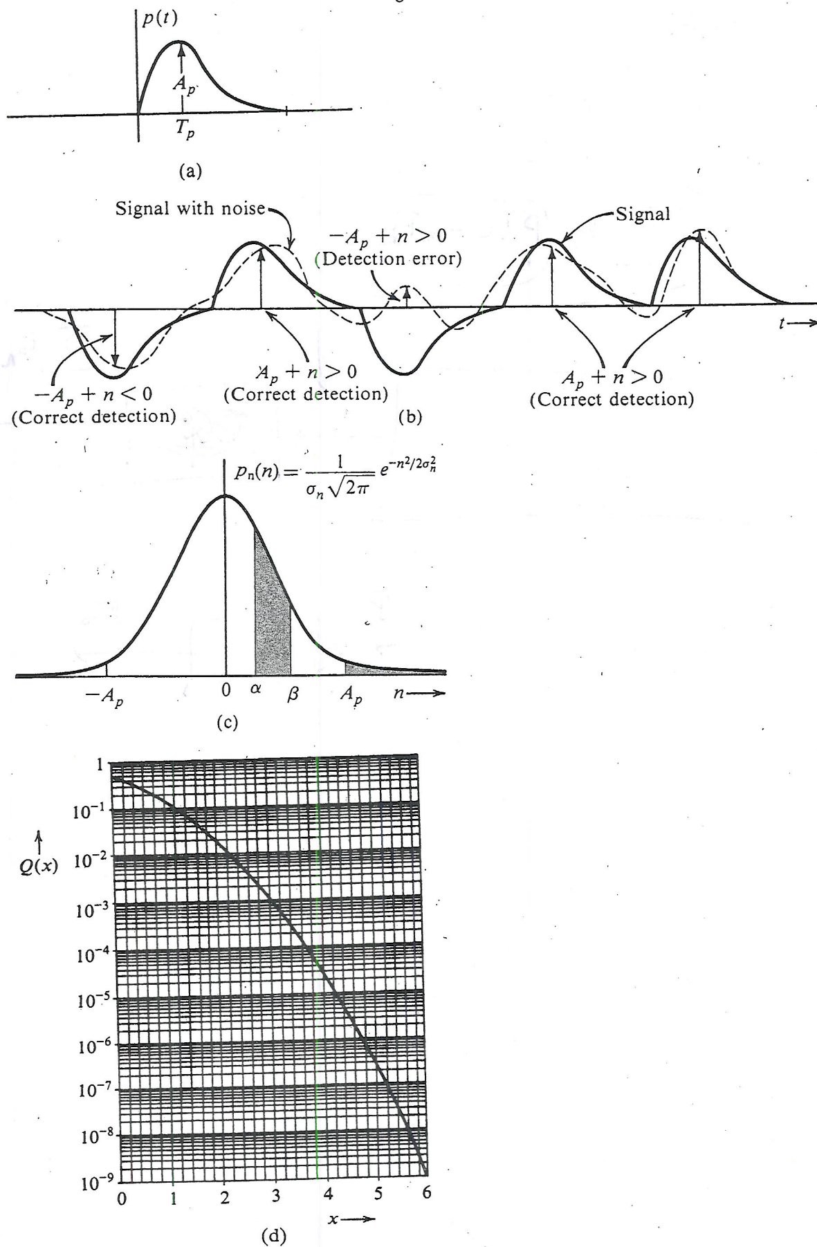
Figure 10.11 Error probability in threshold detection.
