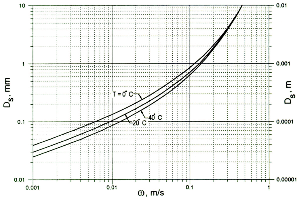
Figure 5.8. Fall velocity of sand-sized particles with specific gravity of 2.65 in metric units.
