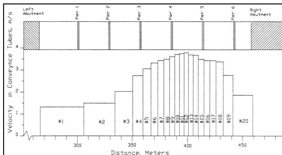
Figure 8.5. Velocity distribution at bridge crossing.
