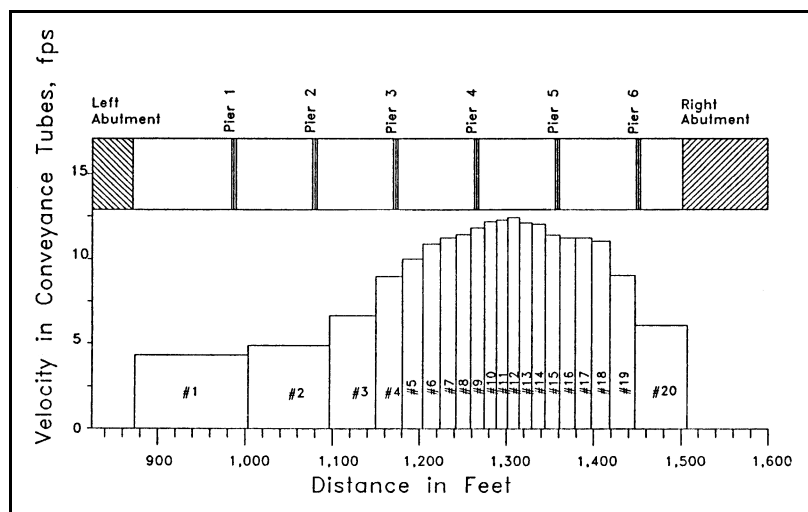
Figure H.5. Velocity distribution at bridge crossing.
