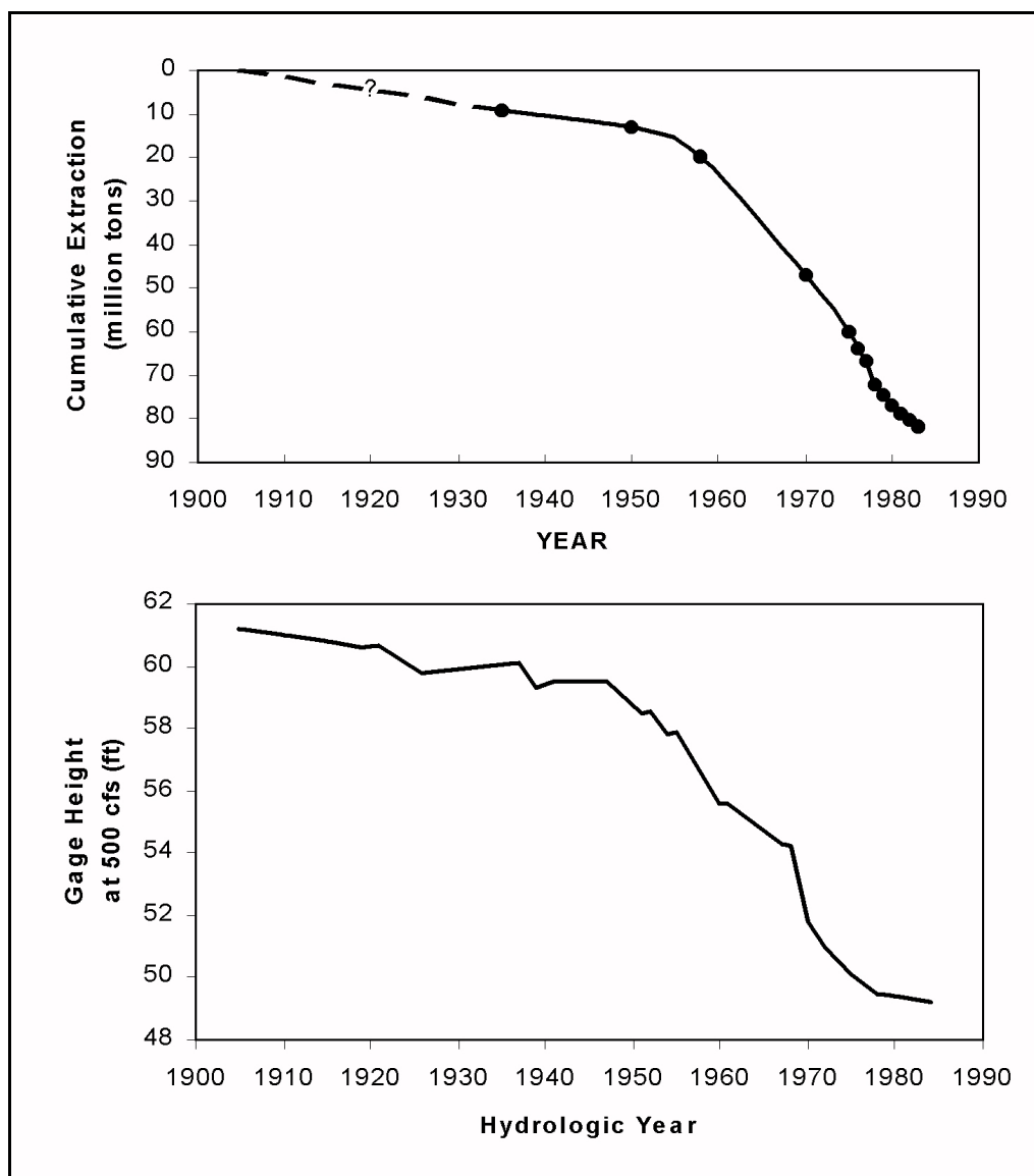
Figure 4.1. Specific gage data for Cache Creek, California.
