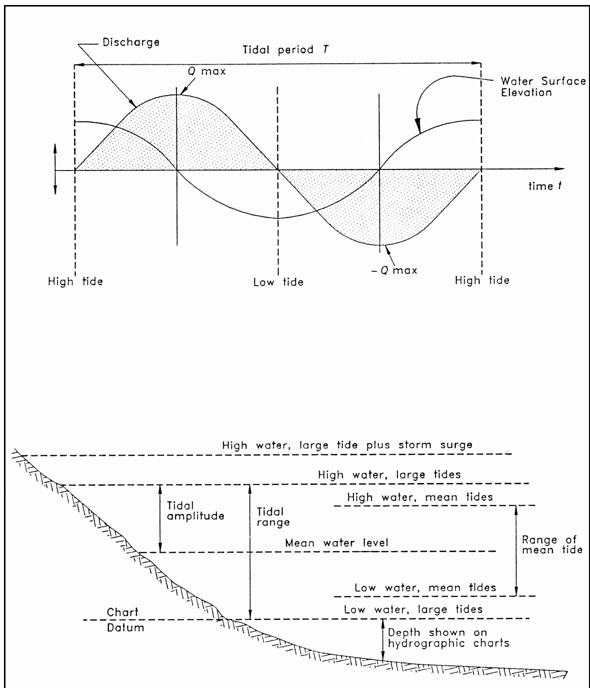
Figure 9.2. Principal tidal terms (after Neill). (78)
