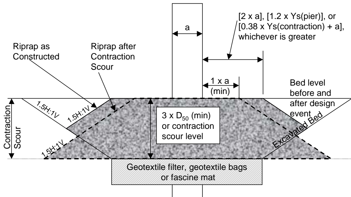
Figure J.2. Riprap design using excavation only.
