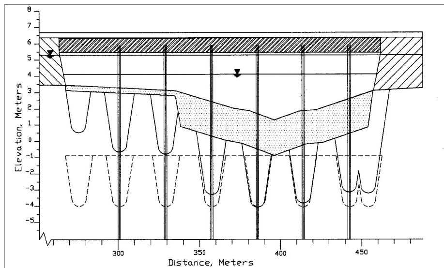
Figure 8.7. Revised plot of total scour for example problem.
