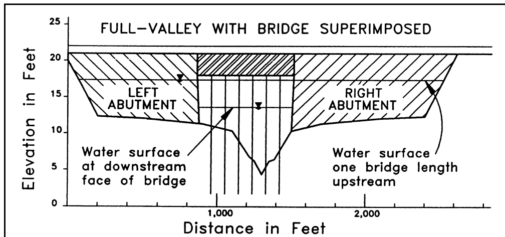
Figure H.1. Cross section of proposed bridge.
