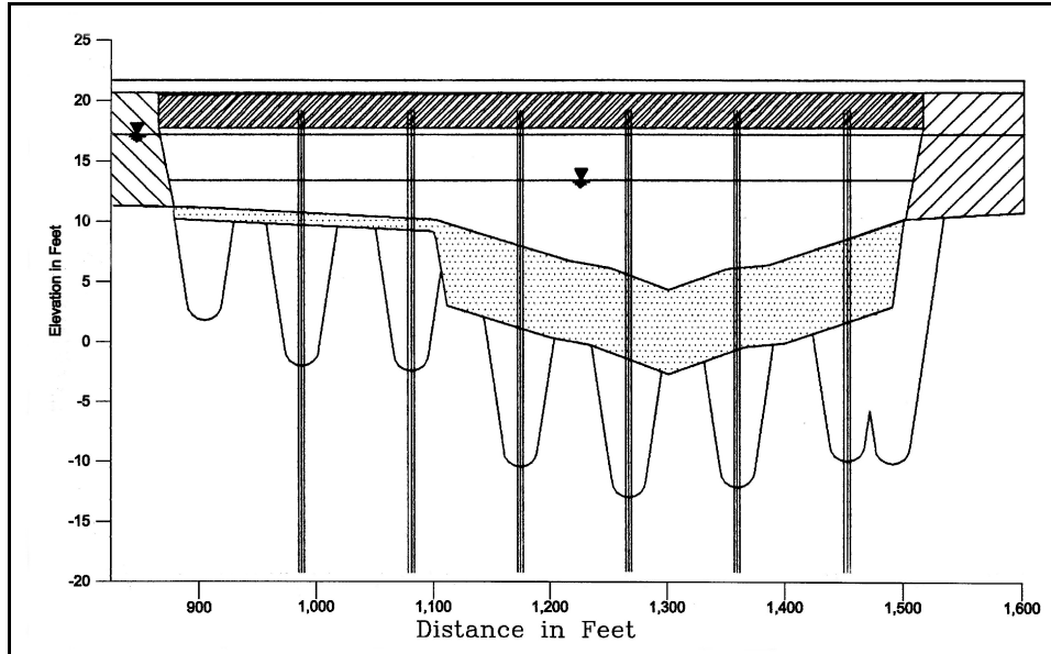
Figure H.6. Plot of total scour for example problem.
