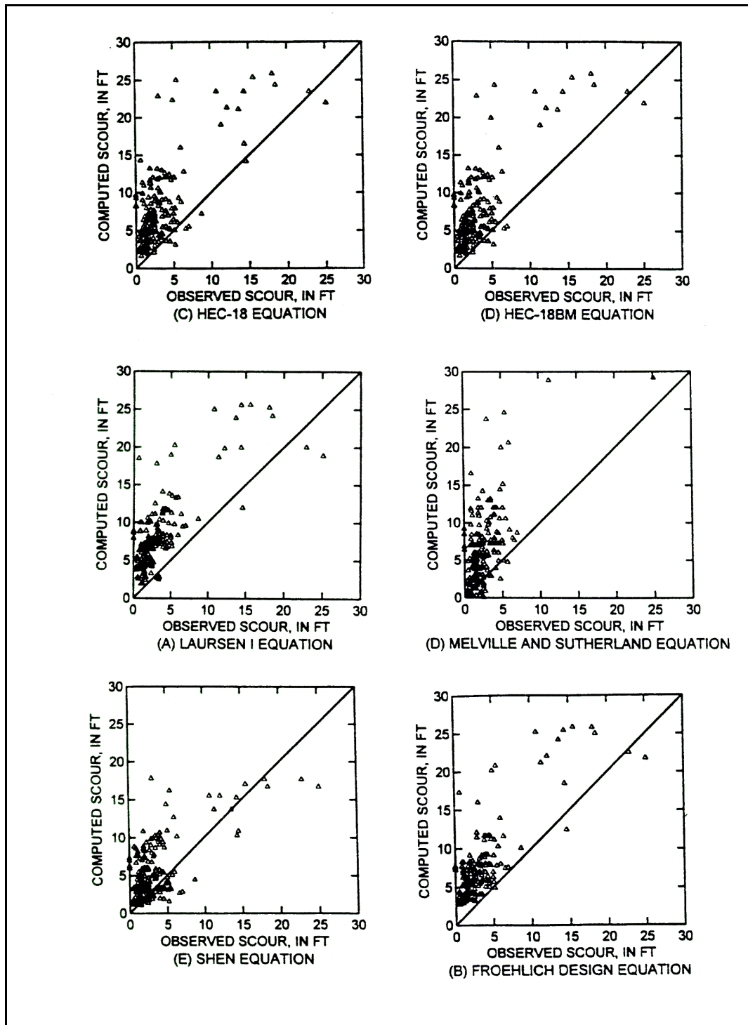
Figure 6.2. Comparison of scour equations with field scour measurements (after Mueller). (49)
