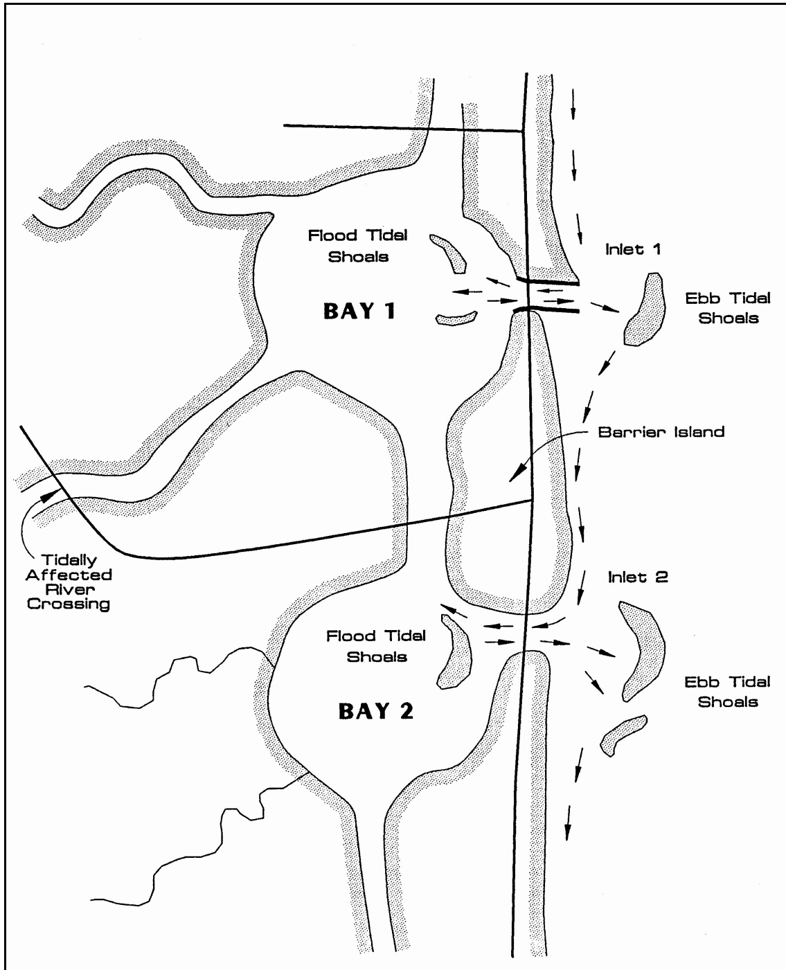
Figure 9.3. Sediment transport in tidal inlets (after Sheppard). (81)
