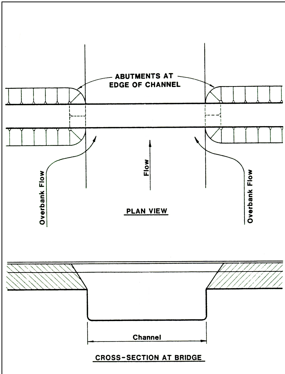
Figure 5.2. Case 1B: Abutments at edge of channel.
