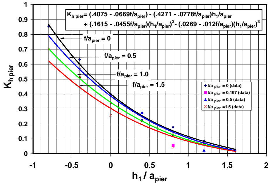
Figure 6.5. Suspended pier scour ratio. (59)
