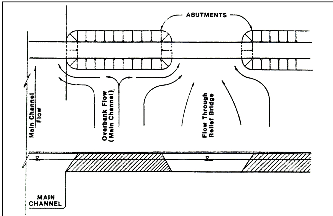
Figure 5.6. Case 3: Relief bridge over floodplain.
