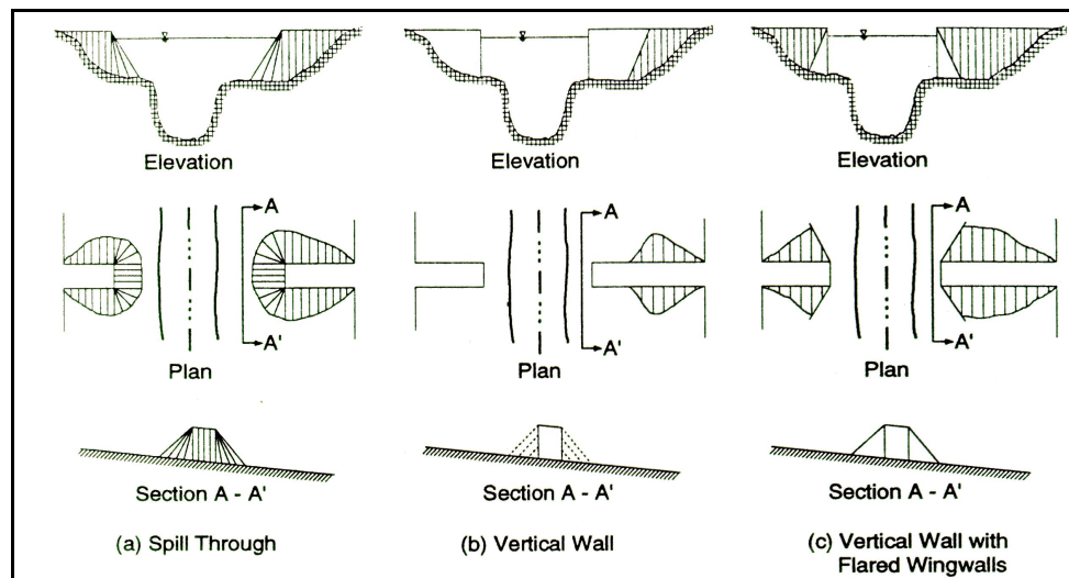
Figure 7.6. Abutment shape.
