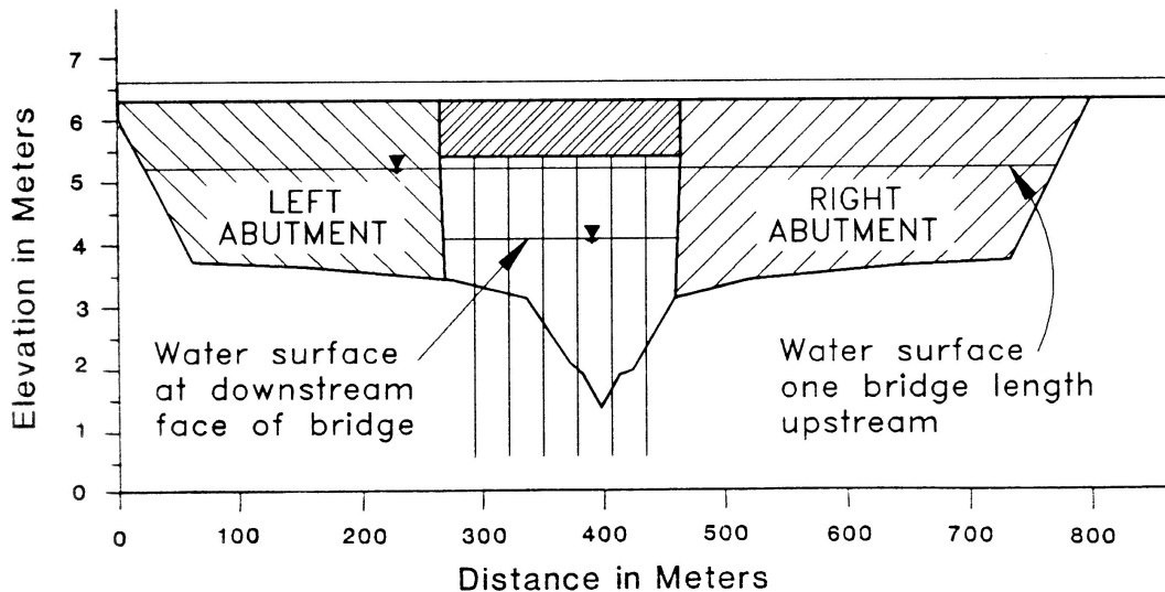
Figure 8.1. Cross section of proposed bridge.
