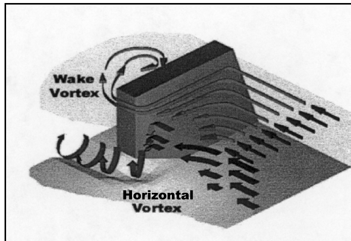
Figure 7.1. Schematic representation of abutment scour.
