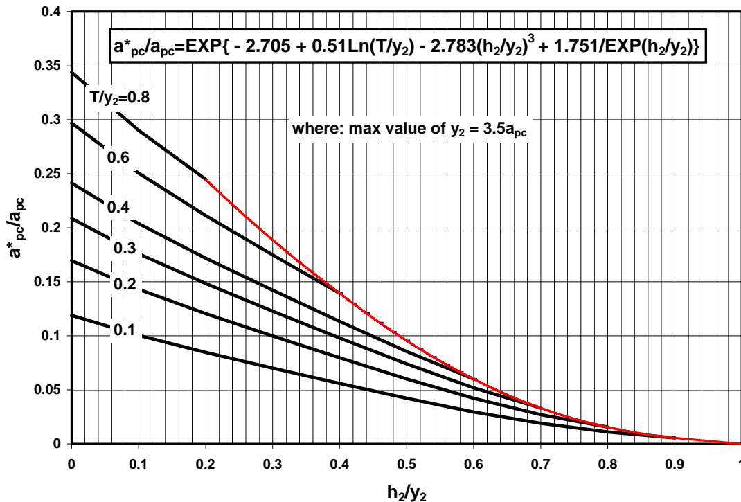
Figure 6.6. Pile cap (footing) equivalent width. (59)
