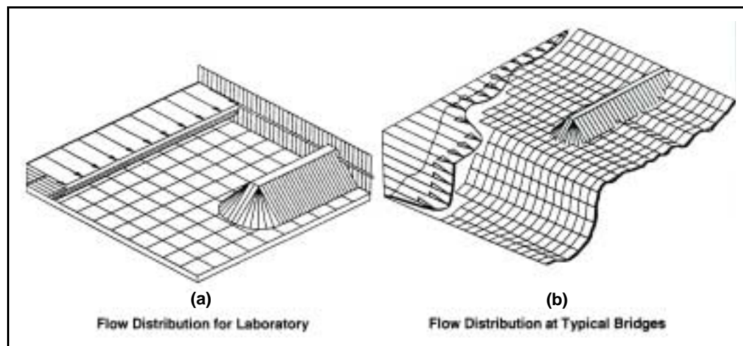
Figure 7.3. Comparison of (a) laboratory flow characteristics to (b) field flow conditions.
