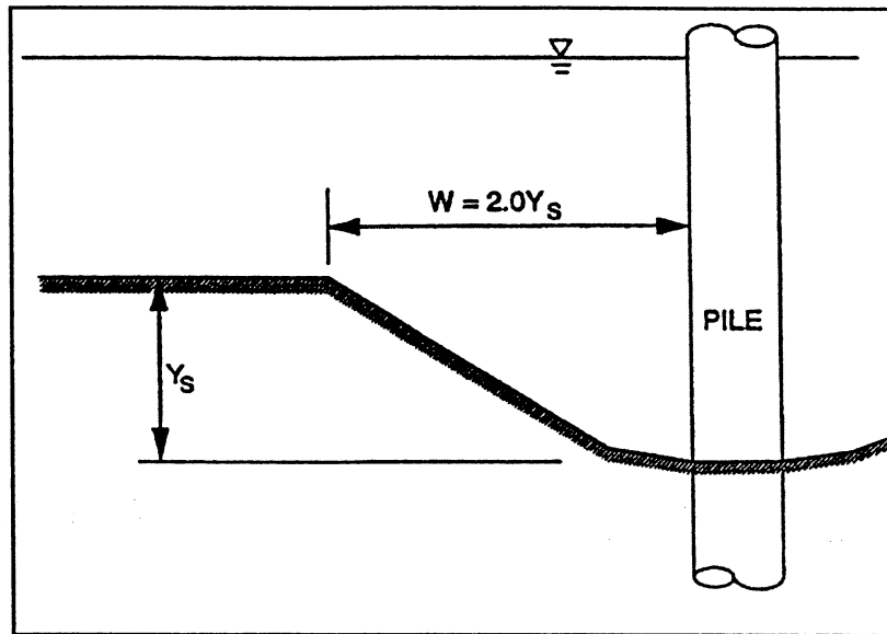
Figure 6.15. Topwidth of scour hole.
