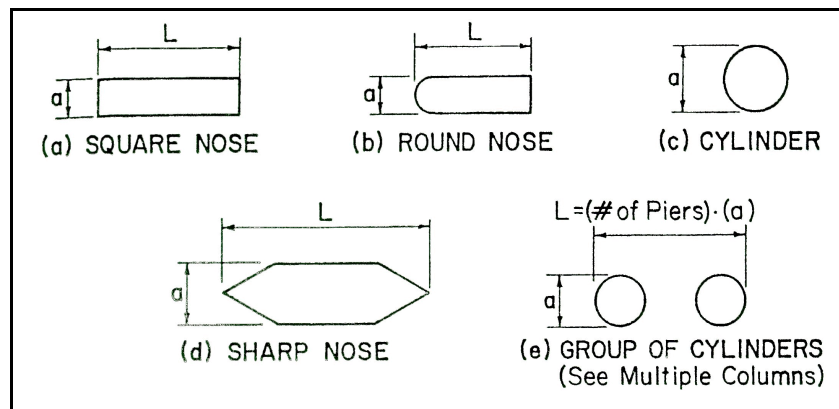
Figure 6.3. Common pier shapes.
