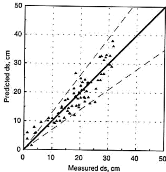
Figure E.1. Comparison of measured and predicted scour depths Sturm Method (1, 2)
