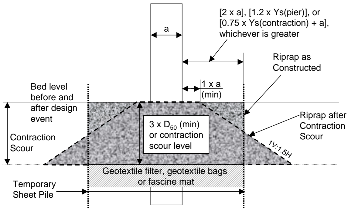
Figure J.1. Riprap design using temporary sheet pile.
