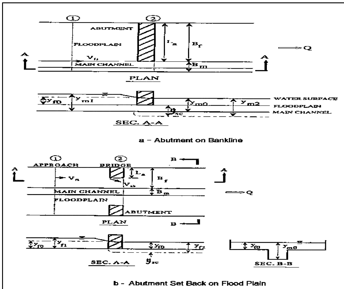
Figure E.2. Definition sketches for application of the Sturm method.
