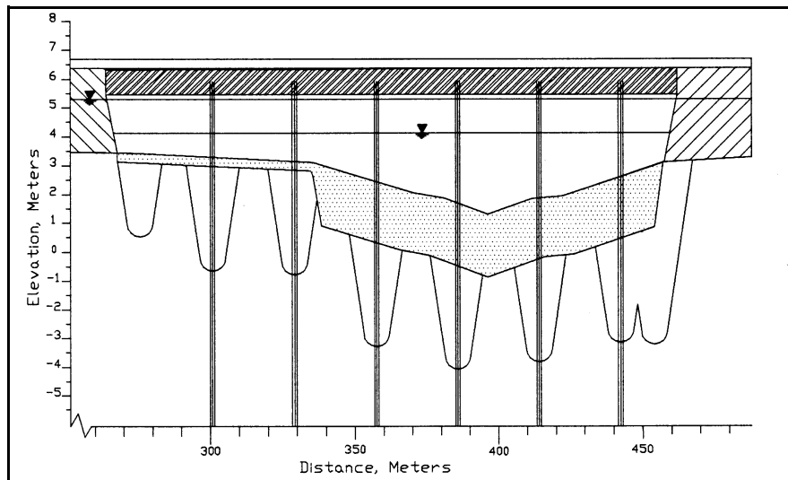
Figure 8.6. Plot of total scour for example problem.
