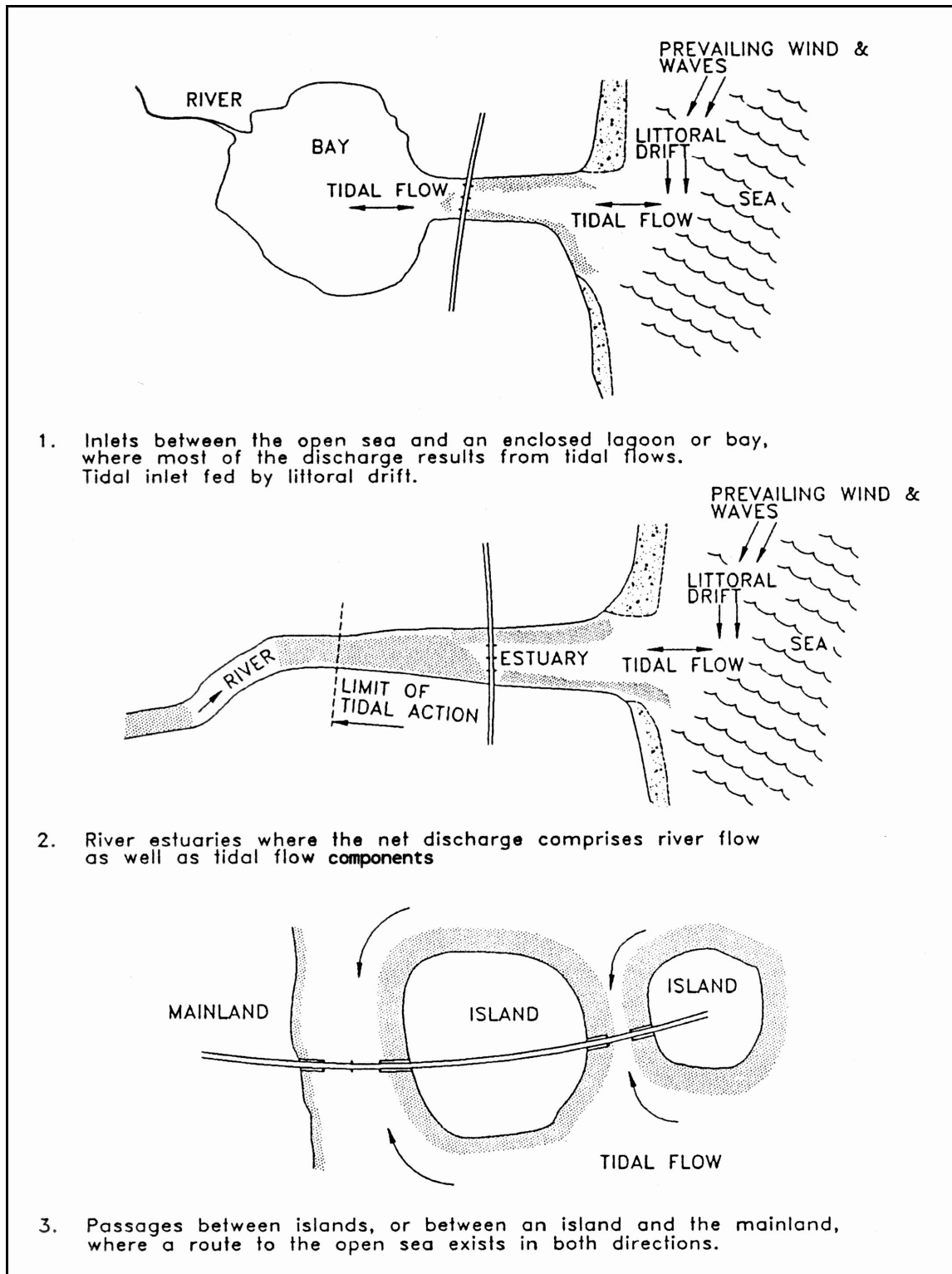
Figure 9.1. Types of tidal waterway crossings (after Neill). (78)
