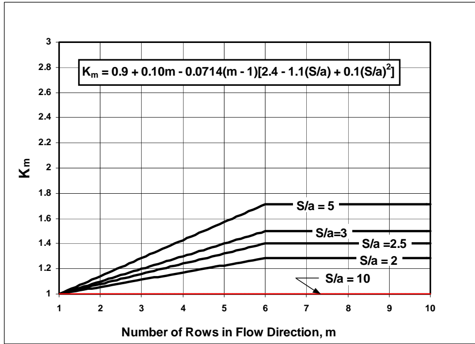
Figure 6.11. Adjustment factor for number of aligned rows of piles (refer to Sheppard). (62)
