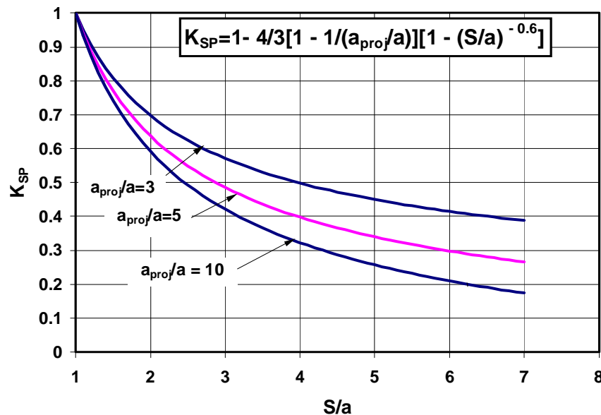
Figure 6.10. Pile spacing factor (refer to Sheppard). (62)
