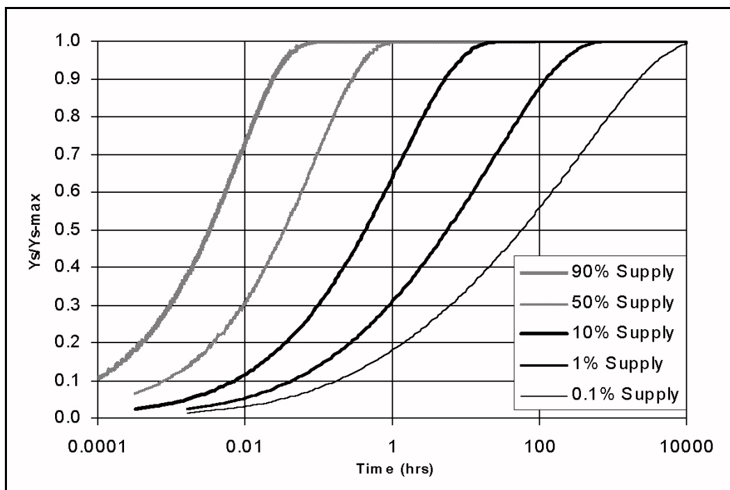
Figure 9.7. Contraction scour development with sediment supply.
