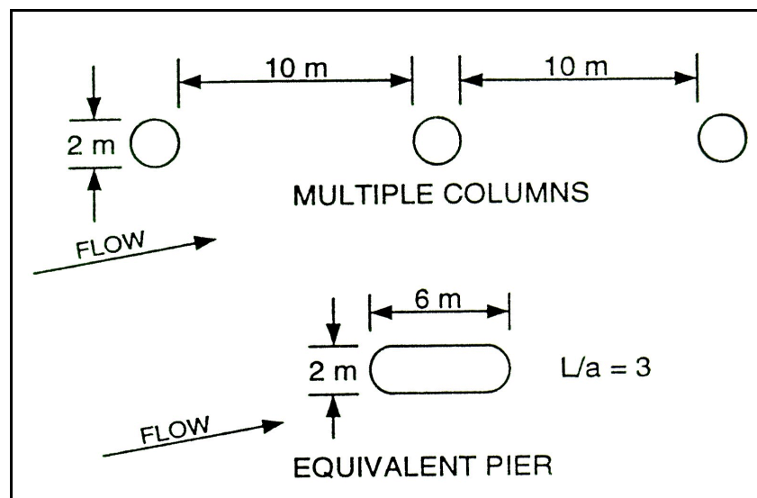
Figure 6.13. Multiple columns skewed to the flow.
