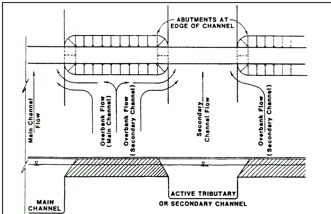
Figure 5.7. Case 4: Relief bridge over secondary stream.
