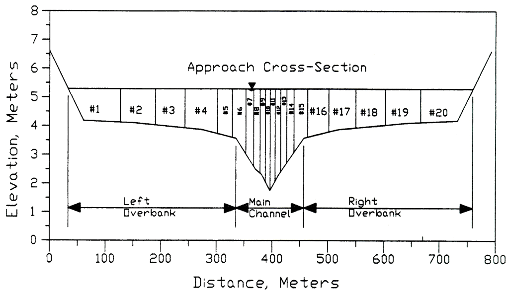
Figure 8.2. Equal conveyance tubes of approach section.
