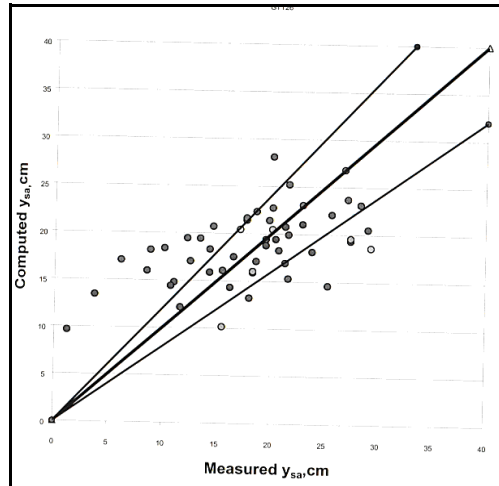
Figure F.2. Comparison of measured and predicted scour depths, Maryland SHA Equations.
