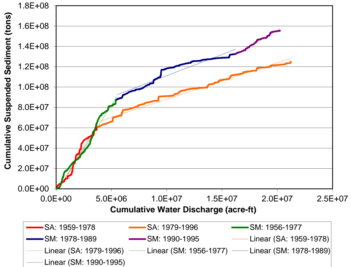
Figure 4.68 Suspended Sediment Concentration Double Mass Curves (Larsen et al. 2007)
