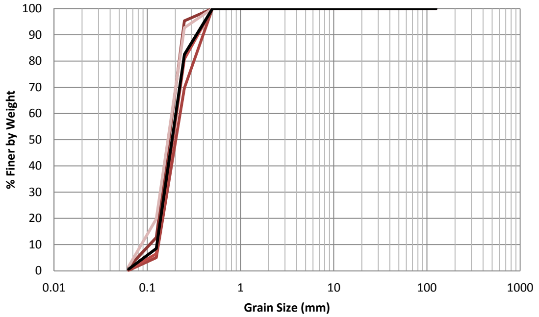
Figure H.21 EB-13 1999 Grain Size Distribution
