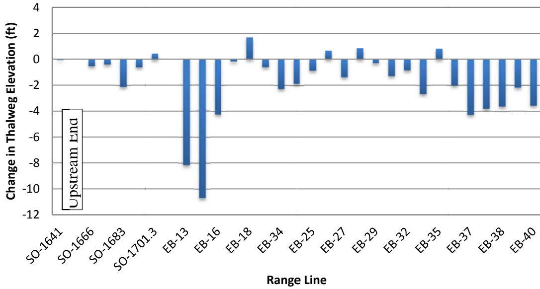
Figure 4.40 Magnitude of Aggradation and Degradation at Range Lines (2003-2004)
