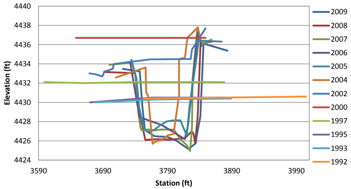
Figure F.26 EB-30 Cross-Section
