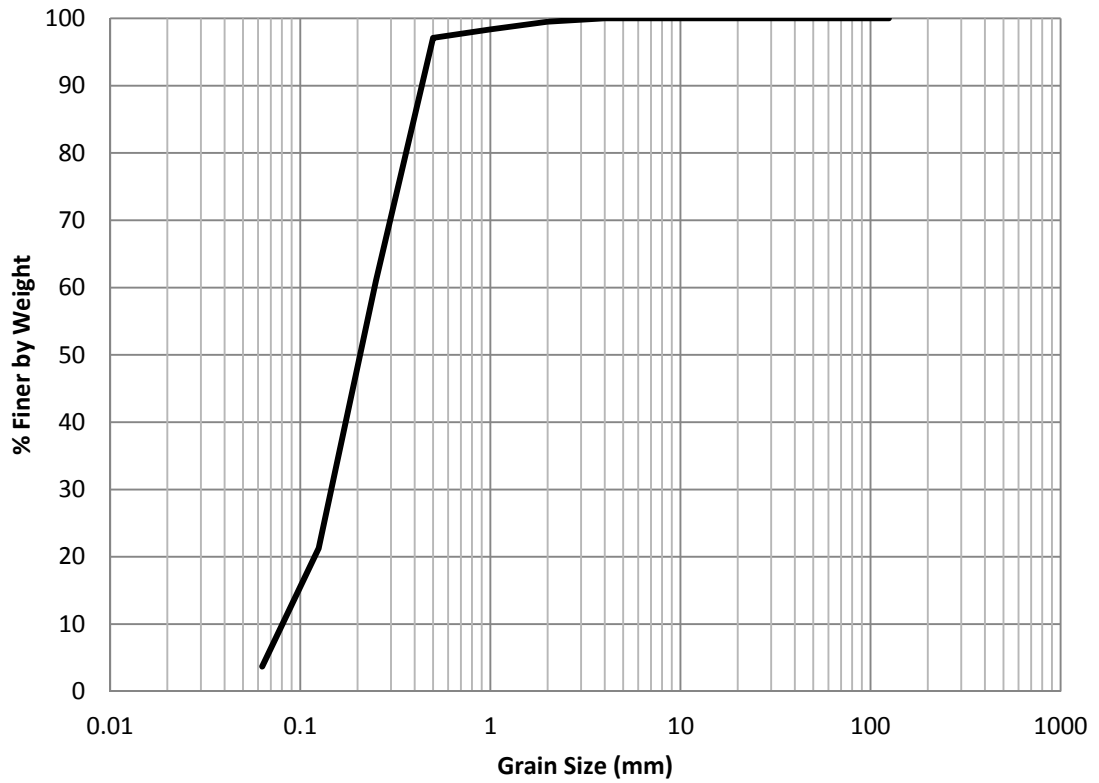
Figure H.21 EB-13 1999 Grain Size Distribution
