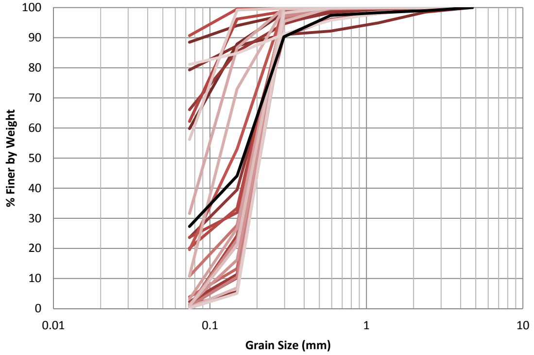
Figure H.23 EB-18 1986 Grain Size Distribution
