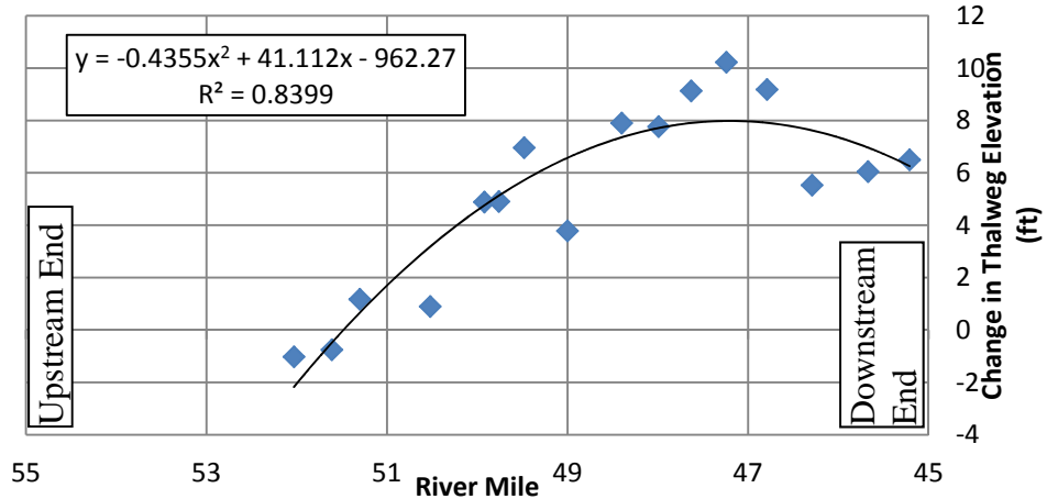
Figure 4.46 Magnitude of Aggradation from 2004-2009
