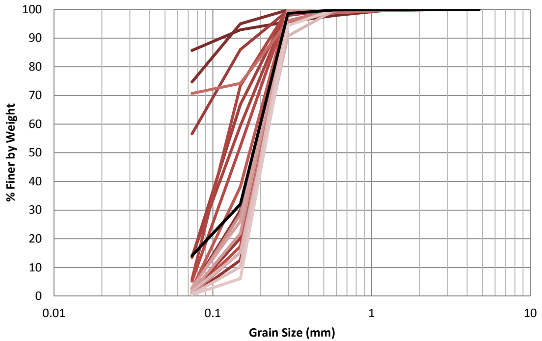
Figure H.17 EB-13 1986 Grain Size Distribution
