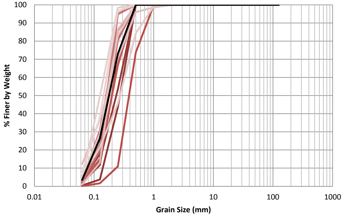
Figure H.27 EB-18 1993 Grain Size Distribution
