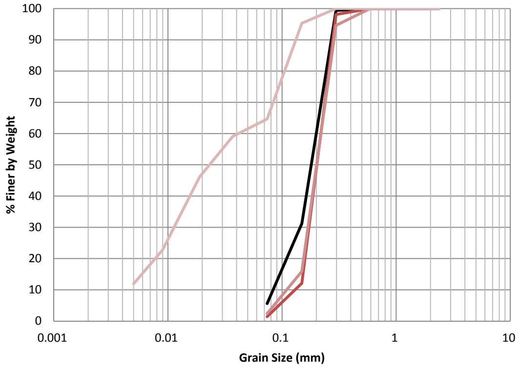
Figure H.9 EB-10 1990 Grain Size Distribution
