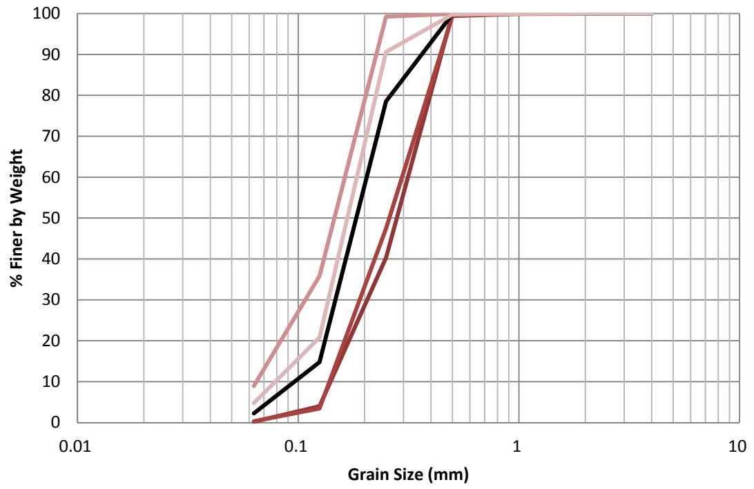
Figure H.5 SO-1683 1999 Grain Size Distribution
