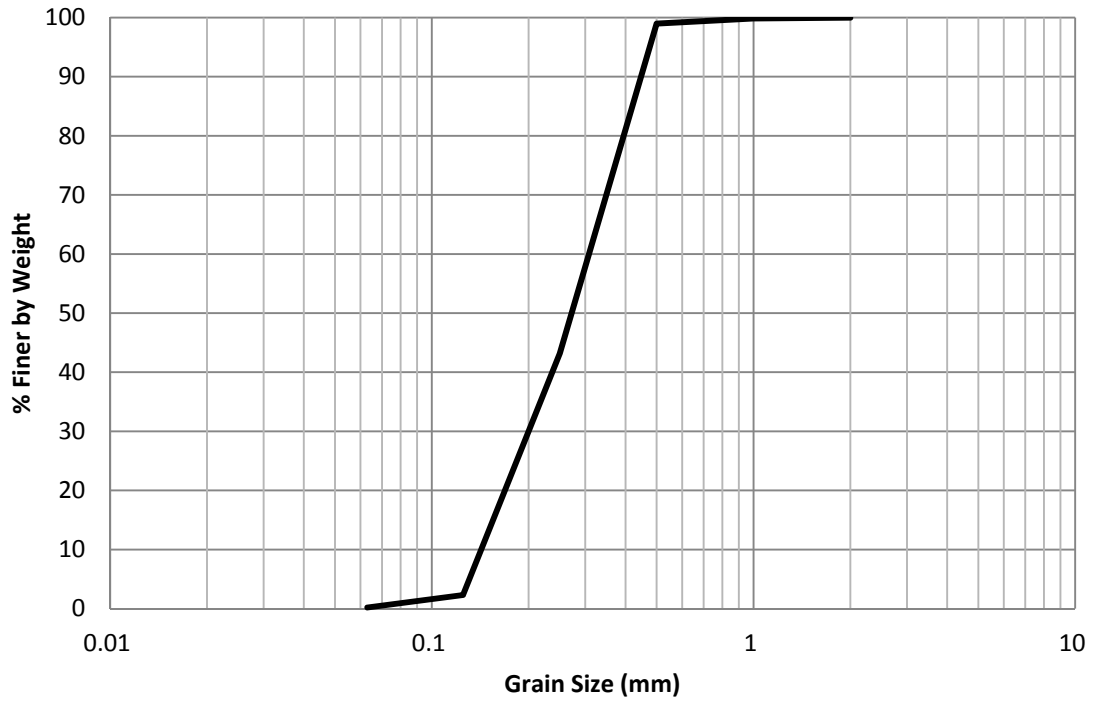
Figure H.1 SO-1641 2001 Grain Size Distribution
