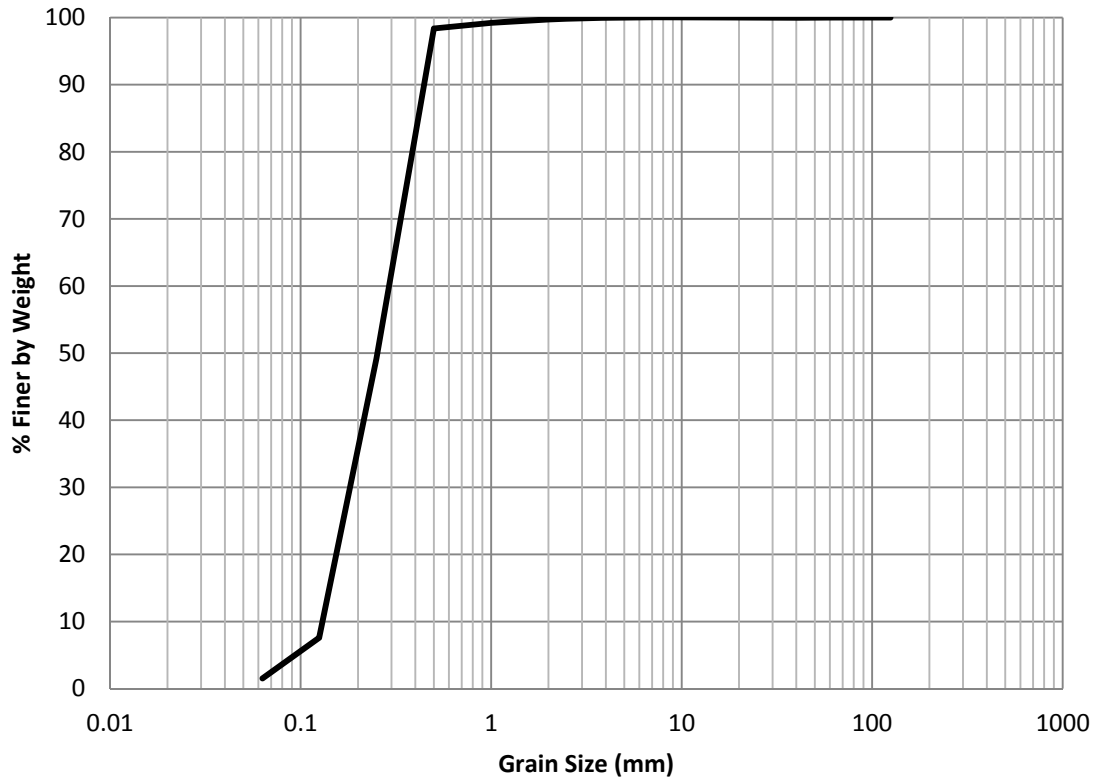
Figure H.31 EB-18 2002 Grain Size Distribution
