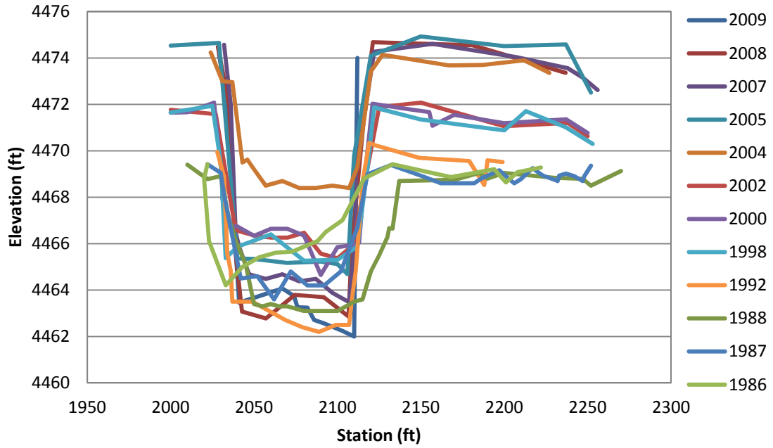
Figure F.10 EB-13 Cross-Section
