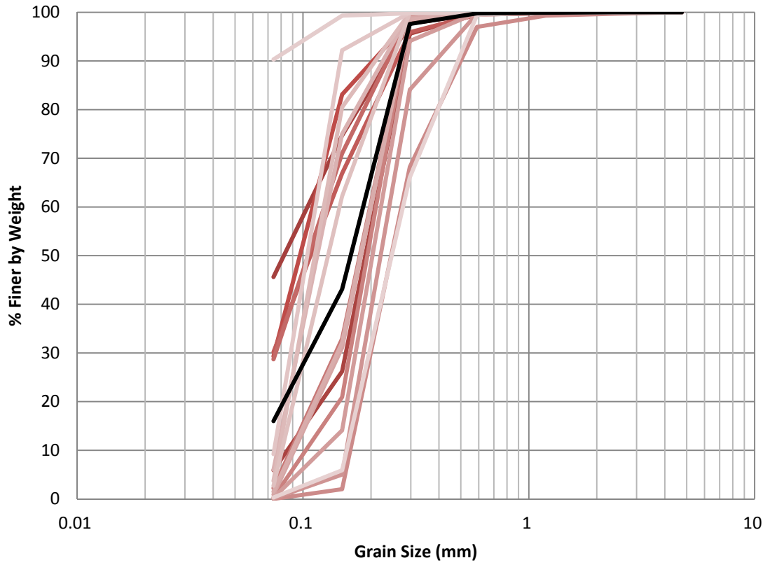
Figure H.6 EB-10 1986 Grain Size Distribution
