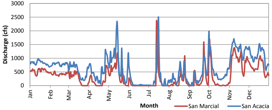
Figure B.1 1990 Daily Discharge Data
