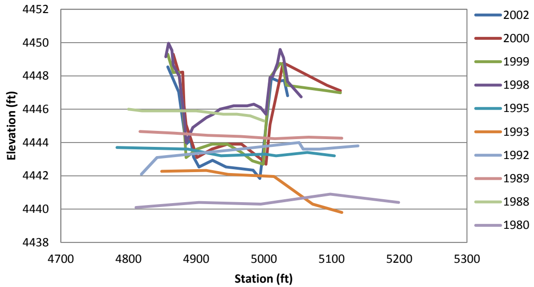
Figure F.20 EB-27 Cross-Section
