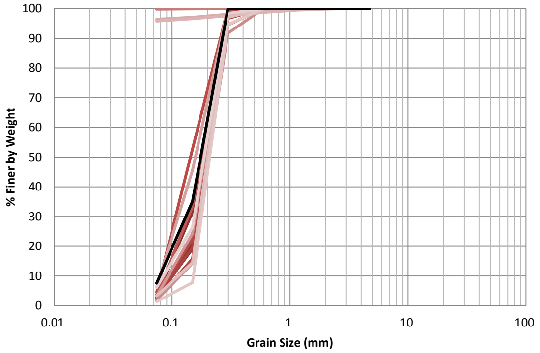
Figure H.7 EB-10 1987 Grain Size Distribution
