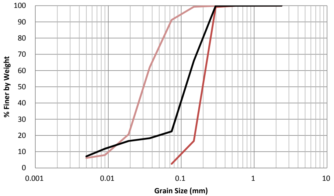
Figure H.19 EB-13 1988 Grain Size Distribution
