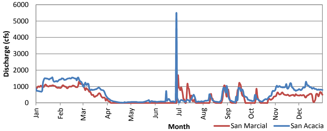
Figure B.7 1996 Daily Discharge Data
