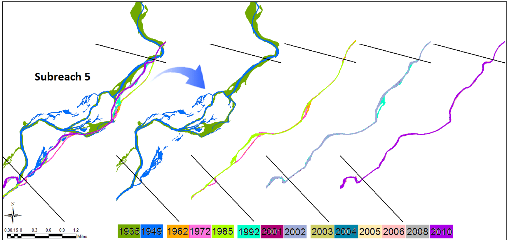
Figure 4.6 Subreach 5 Channel Planforms from Aerial Photography
