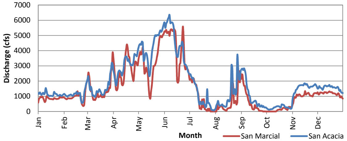
Figure B.4 1993 Daily Discharge Data
