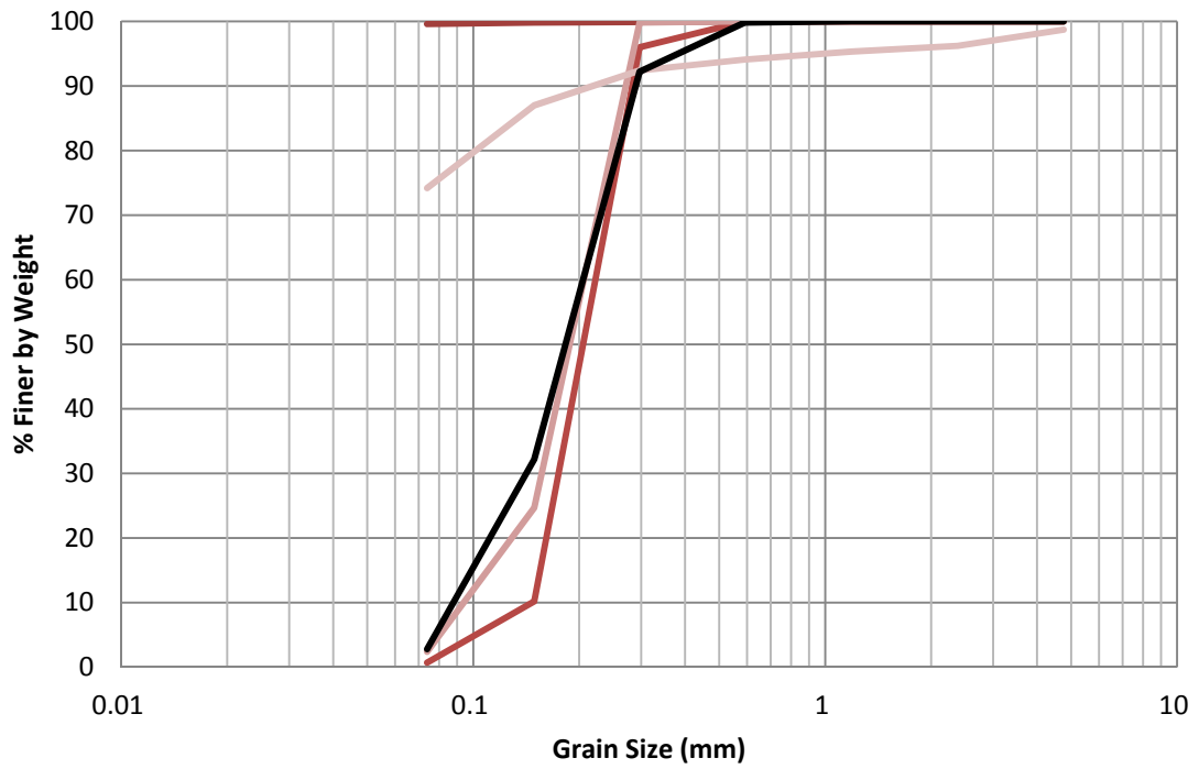
Figure H.7 EB-10 1987 Grain Size Distribution
