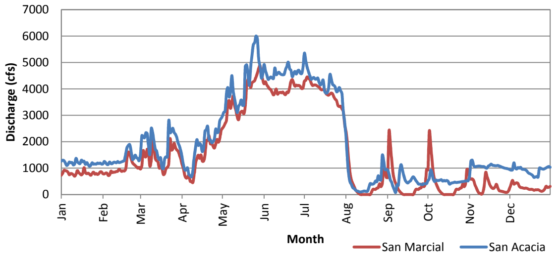
Figure B.6 1995 Daily Discharge Data
