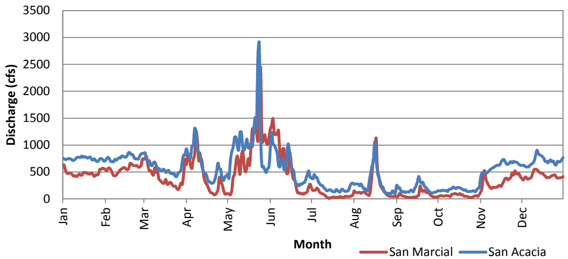
Figure B.12 2001 Daily Discharge Data
