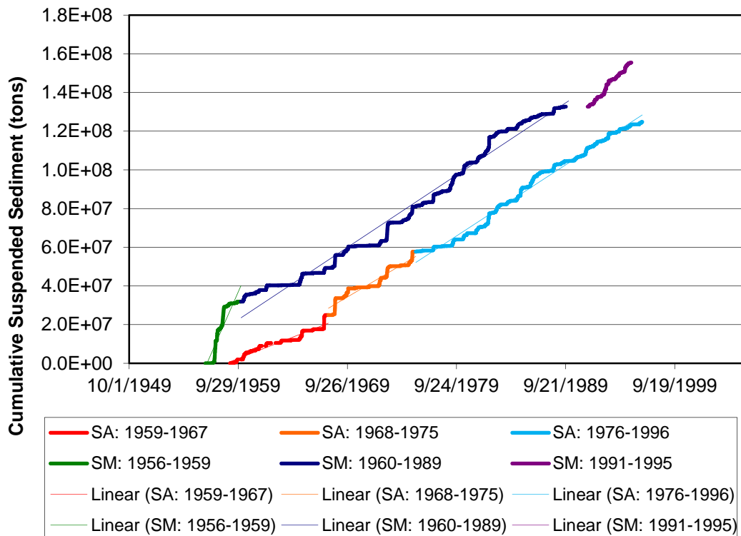
Figure 4.67 Suspended Sediment Discharge Single Mass Curve (Larsen et al. 2007)
