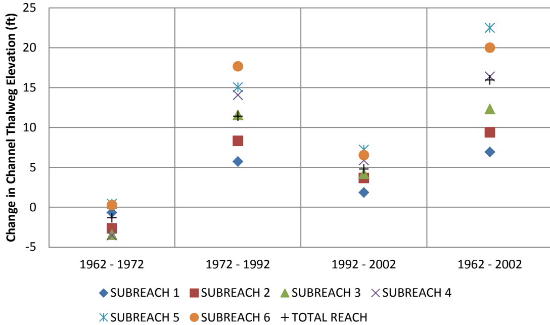
Figure 4.14 Change in Channel Thalweg Elevation from Agg/Deg Surveys
