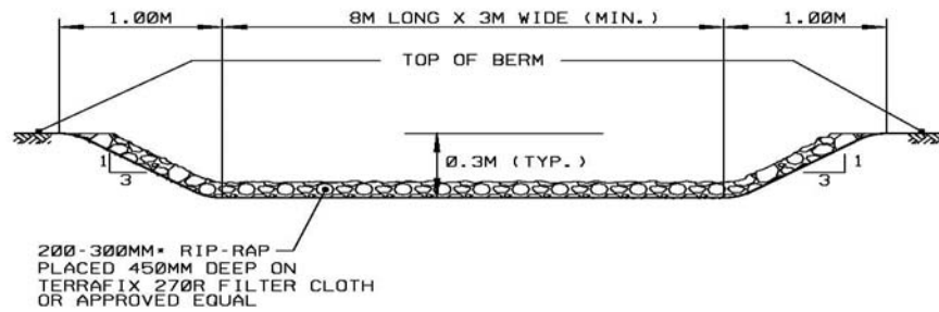
SECTION B-B EMERGENCY WEIR
