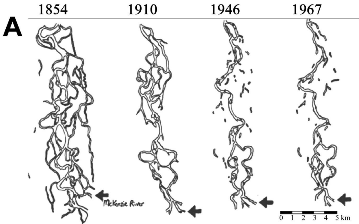
Figure 4-7. (A) Historic Changes to the Upper Willamette Transforming the Natural Anabranching Morphology into a Single-Thread Channel; (B) Lower Taiya River, a Wood-Rich Anabranching River in Southeastern Alaska
