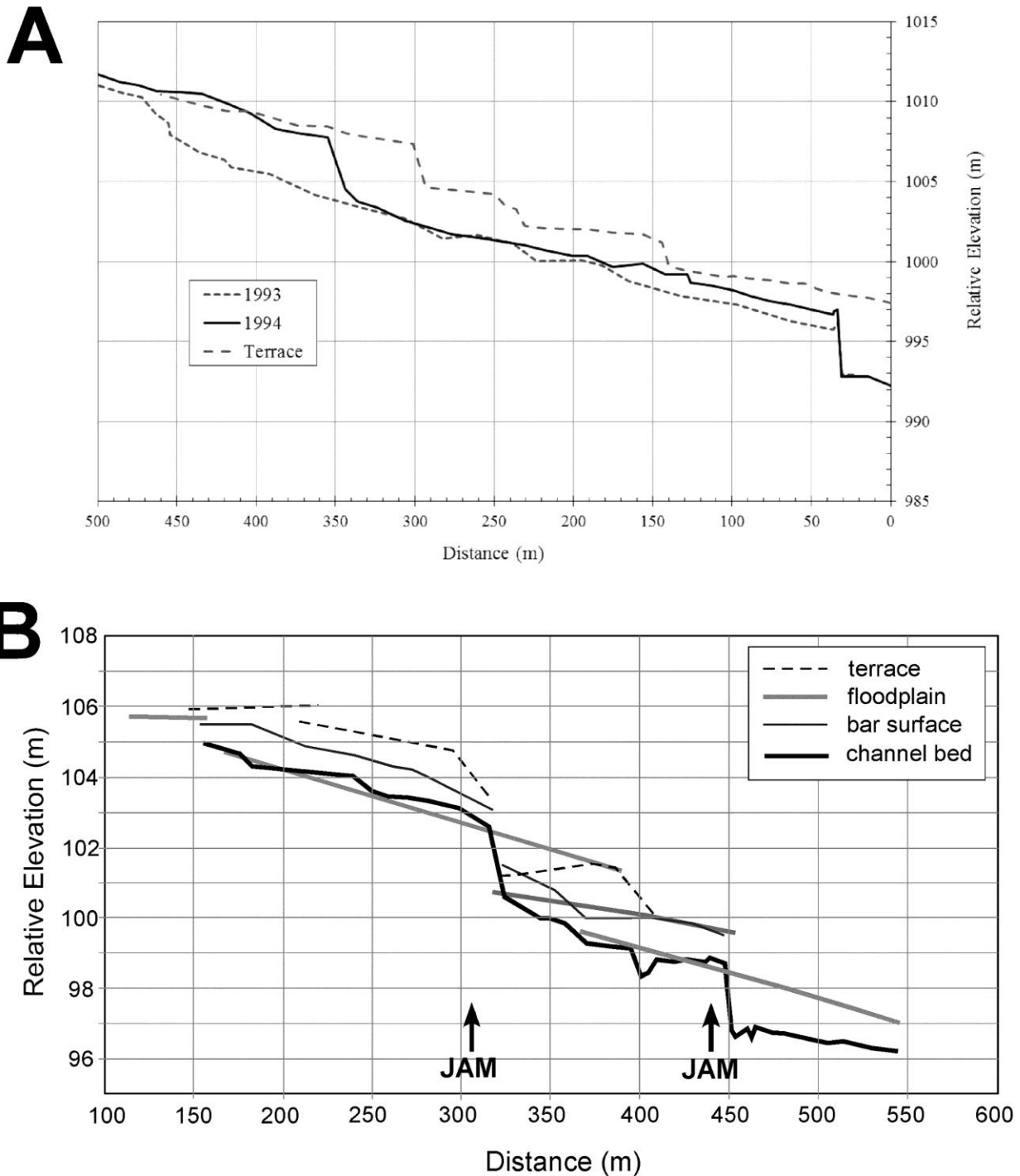
Figure 4-33. Natural Logjam Influence on Channel Aggradation and Terrace Construction in 4 th Order Alta Creek (A) and 6 th Order Mainstem Queets River (B)
