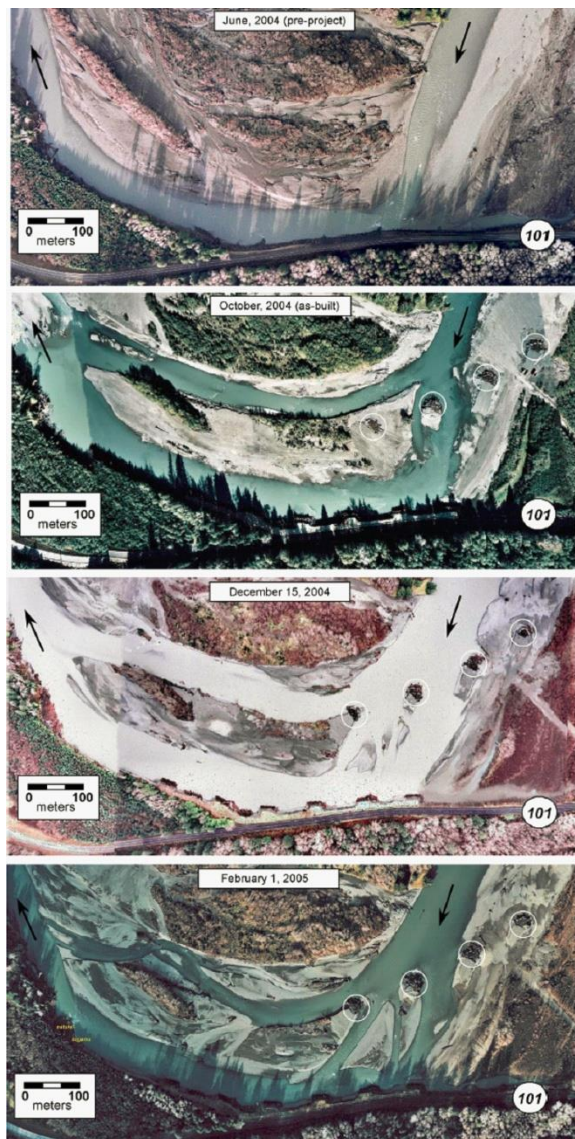
Figure 6-8. Example of the Use of Two Sets of ELJs in Bank Protection Along Hoh River
