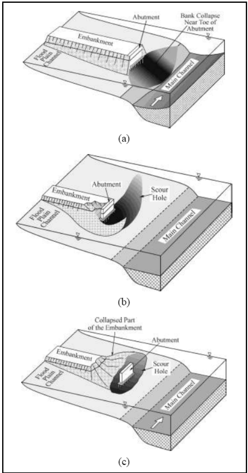
Figure 8.7. Abutment scour conditions (NCHRP 2010b).
