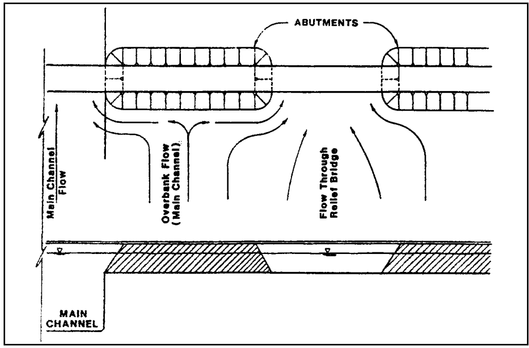
Figure 6.6. Case 3: Relief bridge over floodplain.
