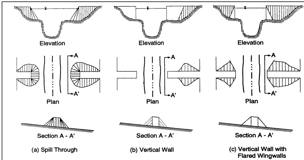
Figure 8.6. Abutment shape.
