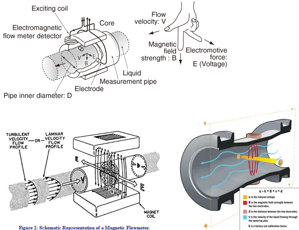
Figure 2: Schematic Representation of a Magnetic Flowmeter.
