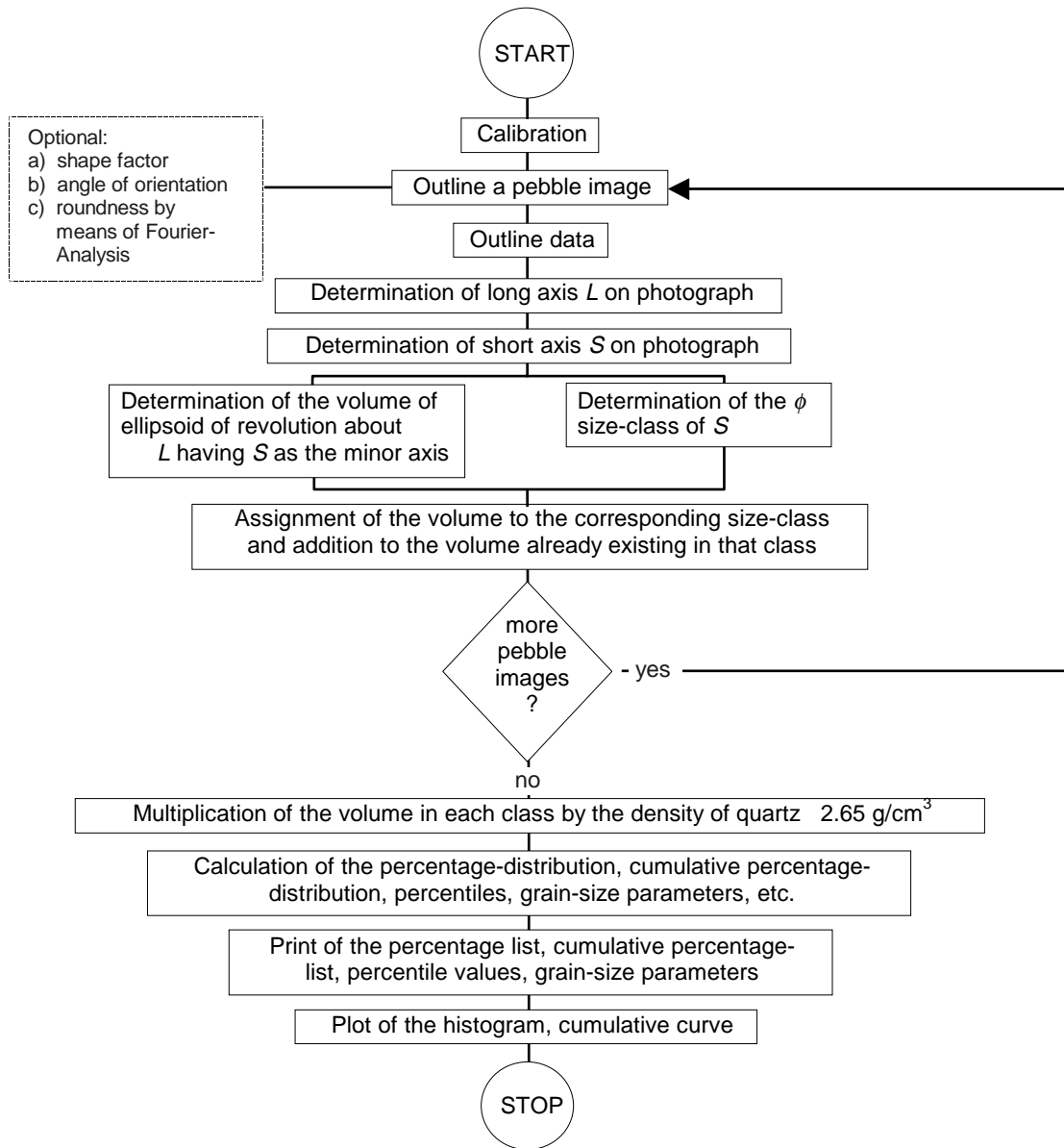
Fig. 4.12: Flow chart for photo sieving analysis. (Redrawn from Ibbeken and Schleyer (1986), by permission of John Wiley and Son. Ltd.).
