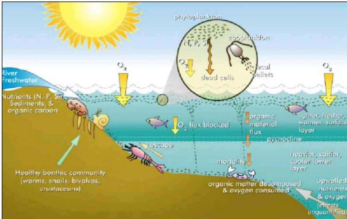
Figure 35: Water quality processes in the delta area of the Mississippi River. Source: U.S. Environmental Protection Agency
