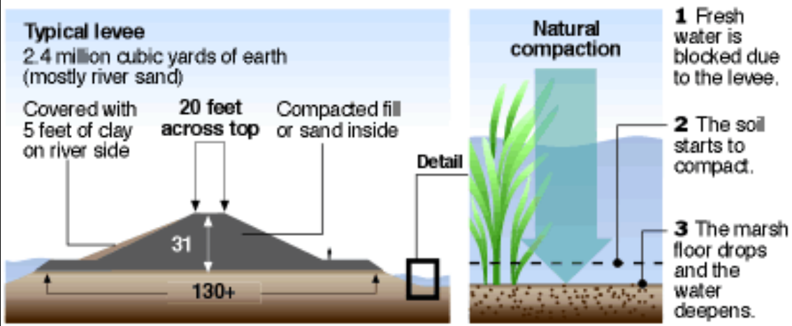
Figure 32: Wetland subsidence cycle and causes
